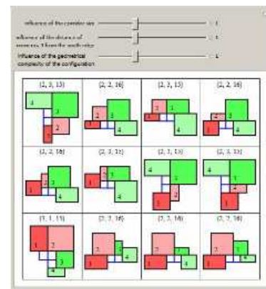
Figure 24. Multi-objective Optimization Tool for Room Configuration.
