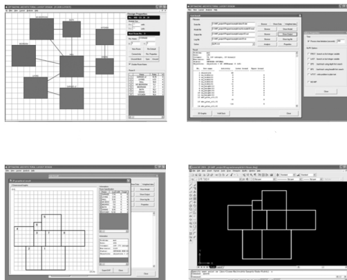
Figure 15. Keatruangkamala and Sinapiromsaram (2005). Mixed Integer Programming.
